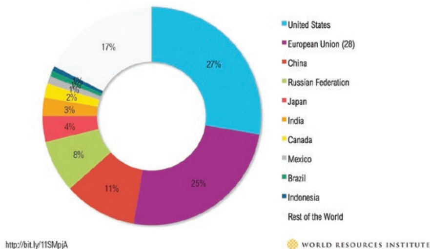
Cumulative CO 2 Emissions 1850–2011 (% of World Total)
