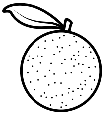
an orange
