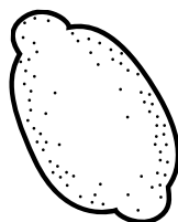
a lemon
