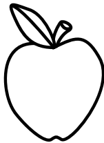
an apple
