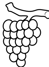
a grape
