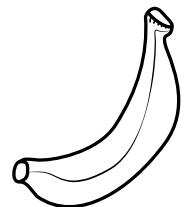
a banana
