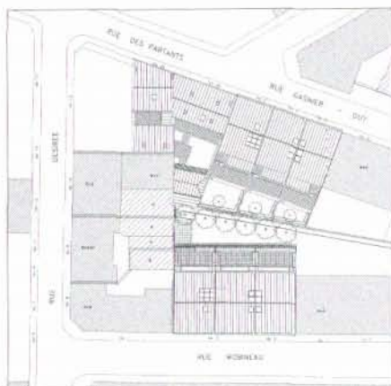
Plan-masse
