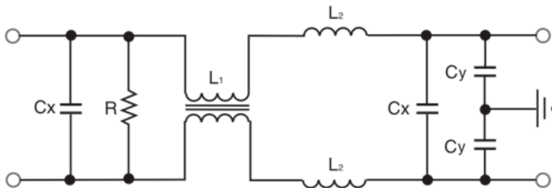
Figure 19: Typical structure of power supply EMC filters
